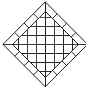
DIAMOND OVERALL SIZE: 5' 2'' TIP TO TIP TILE SIZE: 6'' JOINT WIDTH: \frac{1}{2}''
