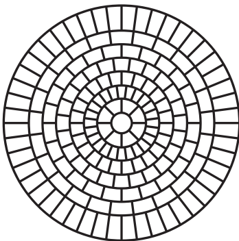
LARGE BRICK ROSETTE DIAMETER: 7' 2'' JOINT WIDTH: \frac{1}{8}''
