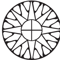
INCA SUN DIAMETER: 2' 11\frac{1}{2}'' JOINT WIDTH: \frac{1}{2}''
