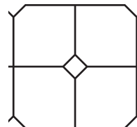
16-INCH DIAMOND TILE LG. TILE SIZE: 16" x 16" INNER TILE: 4" x 4" ROLL WIDTH: 33 1/2" JOINT WIDTH: 1/2"
