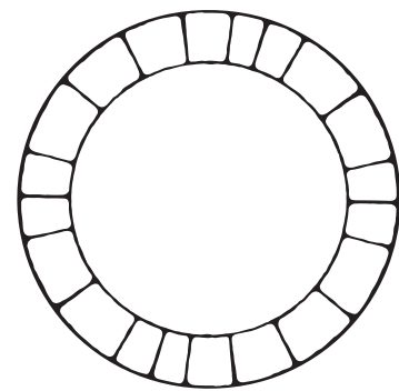
COBBLE CIRCLE RING DIAMETER: 7' 2'' JOINT WIDTH: \frac{1}{2}''
