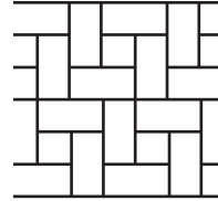
FLANDERS WEAWE FULL BRICK SIZE: 4 1/8" x 10 1/2" ROLL WIDTH: 33" JOINT WIDTH: 1/2"
