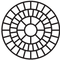
SMALL BRICK ROSETTE DIAMETER: 2' 11\frac{1}{2}'' JOINT WIDTH: \frac{1}{2}''
