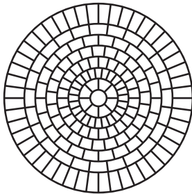
BRICK ROSETTE DIAMETER: 5' 5'' JOINT WIDTH: \frac{1}{2}''
