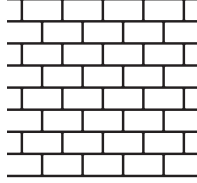
RUNNING BOND BRICK SIZE: 4" x 7 3/4" ROLL WIDTH: 36 1/2" JOINT WIDTH: 1/2"
