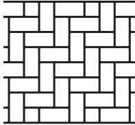
ORIGINAL HERRINGBONE BRICK SIZE: 3 1/2" x 7 3/4" ROLL WIDTH: 33 1/2" JOINT WIDTH: 1/2"
