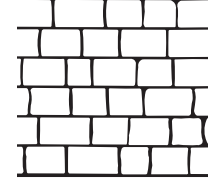
ROMAN PAVER AVERAGE BRICK SIZE: 10" x 5 1/2" ROLL WIDTH: 34" JOINT WIDTH: 1/2"
