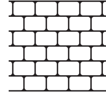
COBBLESTONE BRICK SIZE: 4 3/16" x 7 1/8" ROLL WIDTH: 33" JOINT WIDTH: 1/2"
